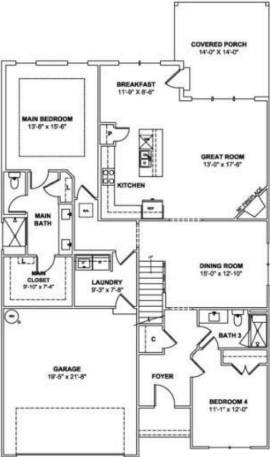
MAIN LEVEL
