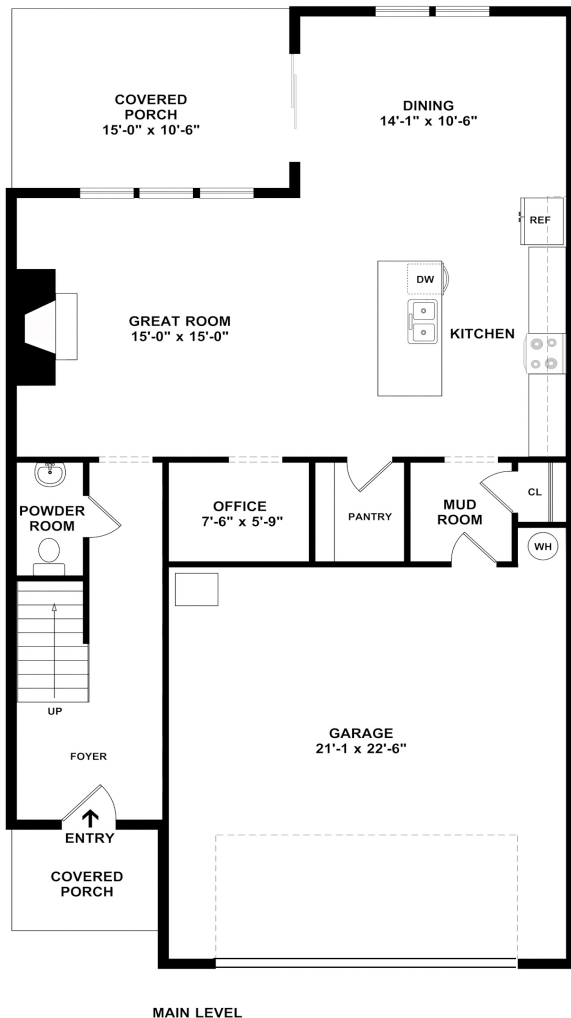
MAIN LEVEL
