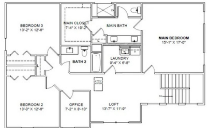
UPPER LEVEL
